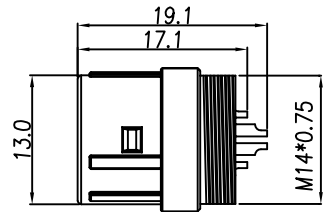
HOUSING+CONTACT+SHELL A
