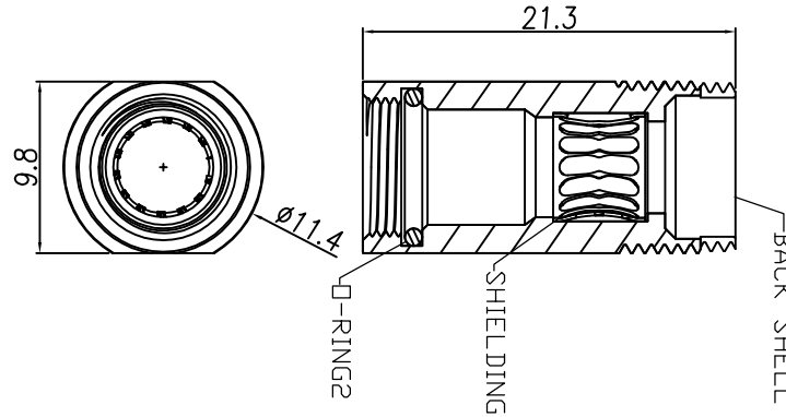
BACK SHELL+SHIELDING+O-RING2
