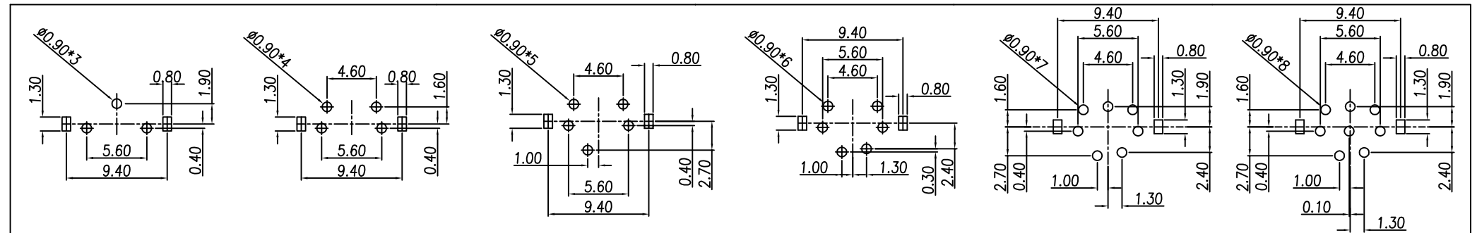
P.C.B LAYOUT (Bottom View)
